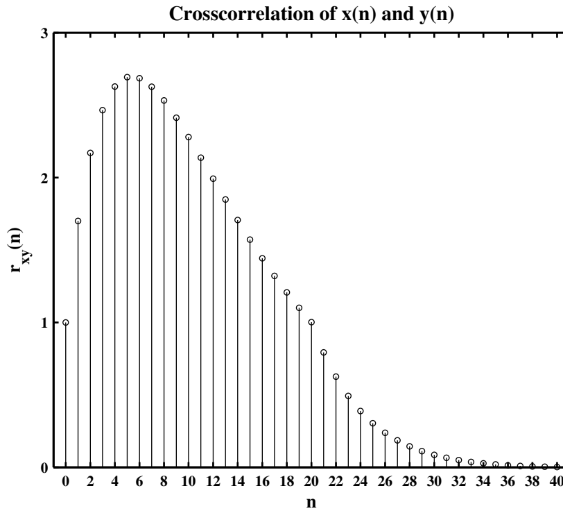
Figure 2.31: Problem P2.9 crosscorrelation plot
