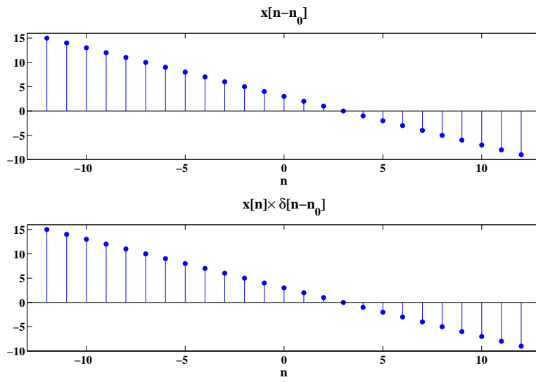
FIGURE 2.39: Verify delay property.
